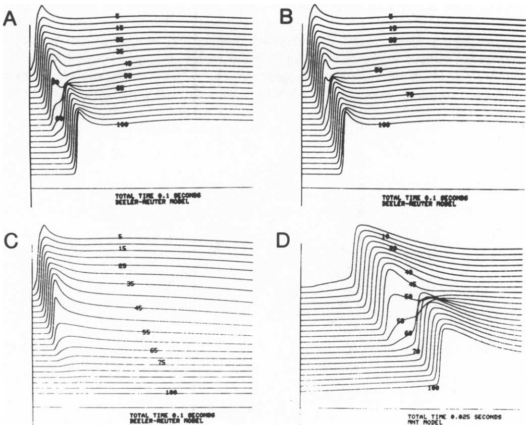
FIGURE 4 ( A ) A series of plots of voltage versus time for 20 segments (5, 10, 15 ... 100) for a 100-segment cable ( \Delta X = 62.5 \mu m ) in which the BR model has \bar{g}_{Na} = 0 for segments 51–56. ( B , C ) Same as A , except that \bar{g}_{Na} = 0 for segments 51–54 ( B ) or 51–58 ( C ). ( D ) Same as A except that MNT membrane model was used and \bar{g}_{Na} = 0 for segments 50–60.
