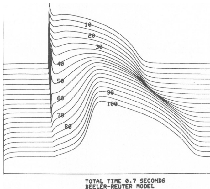
FIGURE 5 A series of plots of voltage versus time for 20 segments (5, 10, 15 ... 100) for a 100-segment cable ( \Delta X = 62.5 \mu\text{m} ) in which the BR model for segments 51-100 was modified with \bar{g}_{Na} = 0 and a depolarization was produced by scaling the background Na current by 2.0 and scaling the background K current by 0.5.
