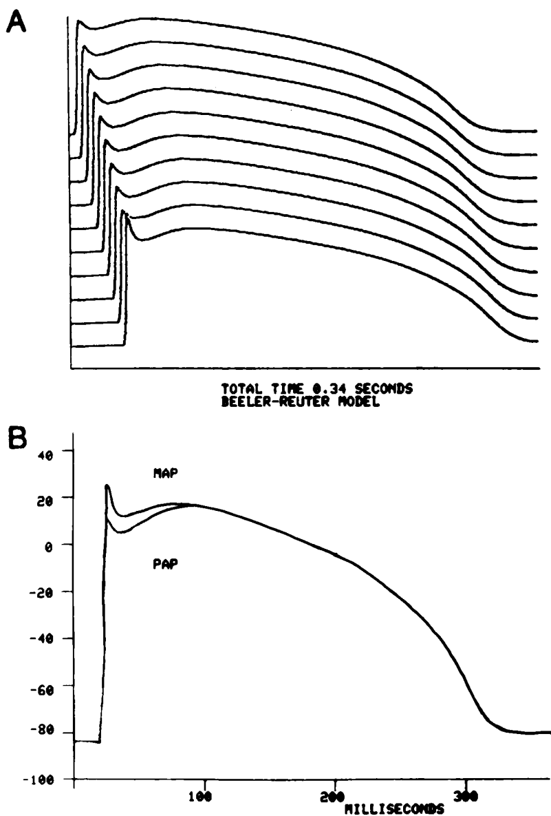
FIGURE 2 (A) A series of plots of voltage versus time for 10 segments (5, 10, 15 . . . 50) for a simulation of the BR model in a strand represented by 50 segments ( \Delta X = 250 \mu\text{m} ). Stimulation occurred at segment 1. Curves are displaced vertically for clarity, with the top trace corresponding to segment 5. (B) The propagating action potential of segment 25 (from A) is superimposed with the isopotential result (MAP) showing the effects of the cable properties in the early part of the AP.
