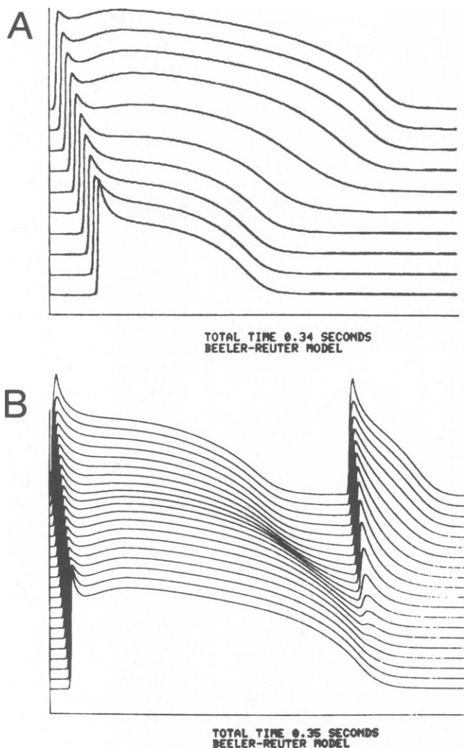
FIGURE 3 ( A ) A series of plots of voltage versus time for 10 segments (5, 10, 15 . . . 50 from top down) for a 50-segment cable in which the BR model has the slow inward current scaled by 1.0 (segments 1-25) or 0.6 (segments 26-50). \Delta X = 250 \mu\text{m} . ( B ) A series of plots of voltage versus time for 20 segments (5, 10, 15 . . . 100 from top down) for a 100-segment cable ( \Delta X = 62.5 \mu\text{m} ) in which the BR model has the slow inward current scaled by 0.1 for segments 1-50 and by 1.0 for segments 51-100. Both stimuli are applied to segment 1.
